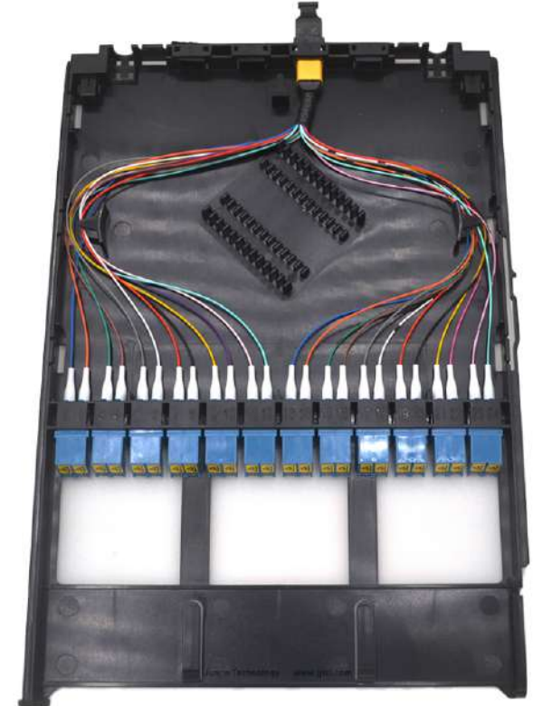
1-MPO-24LC Connection
