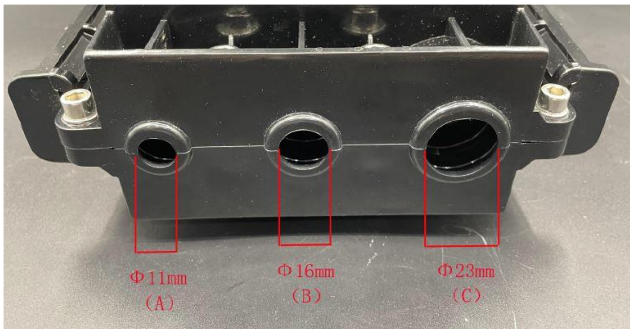
96 Core Optic Splice Joint Closure 3 in 3 out Horizontal Types F003 cable size
